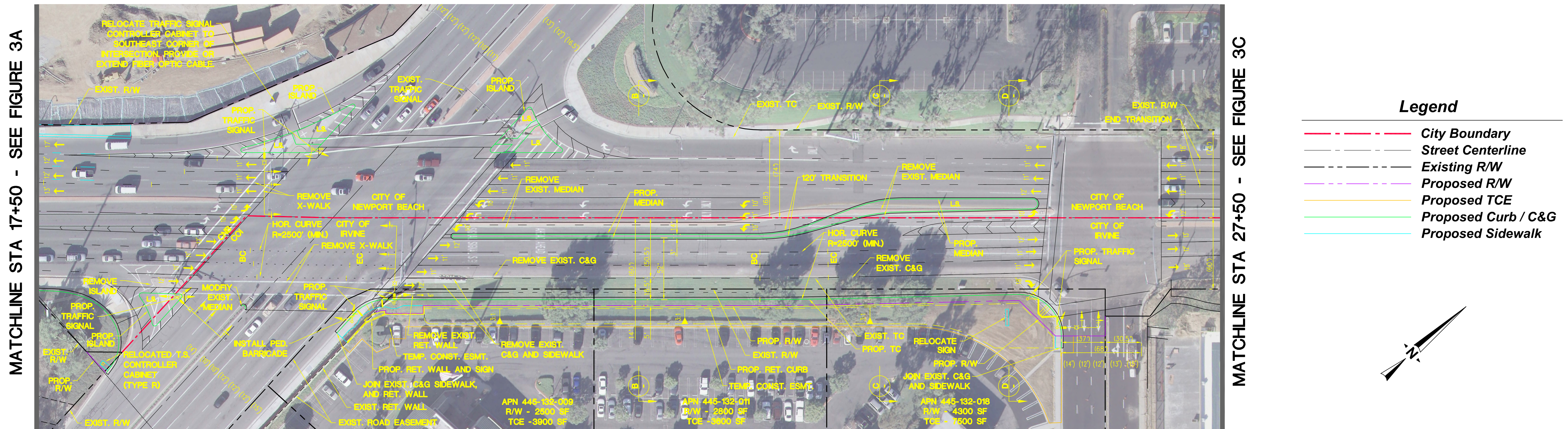
Figure 3B Concept Plan for Jamboree Road Widening
